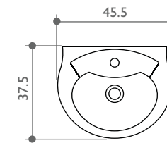
CLOAKROOM BASIN
