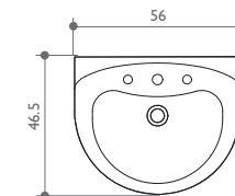
SEMI COUNTERTOP BASIN
