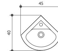
CORNER BASIN
