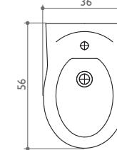
BACK-TO-WALL BIDET
